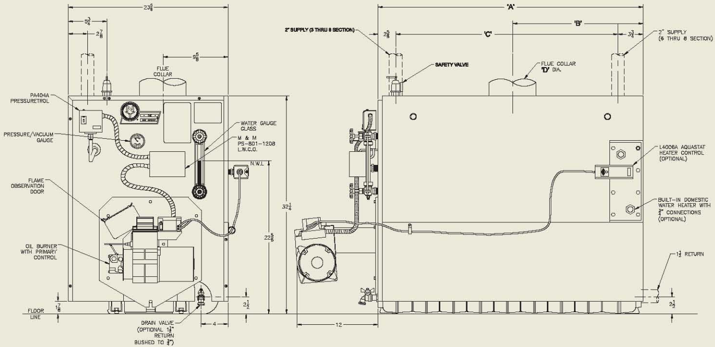
FRONT VIEW
